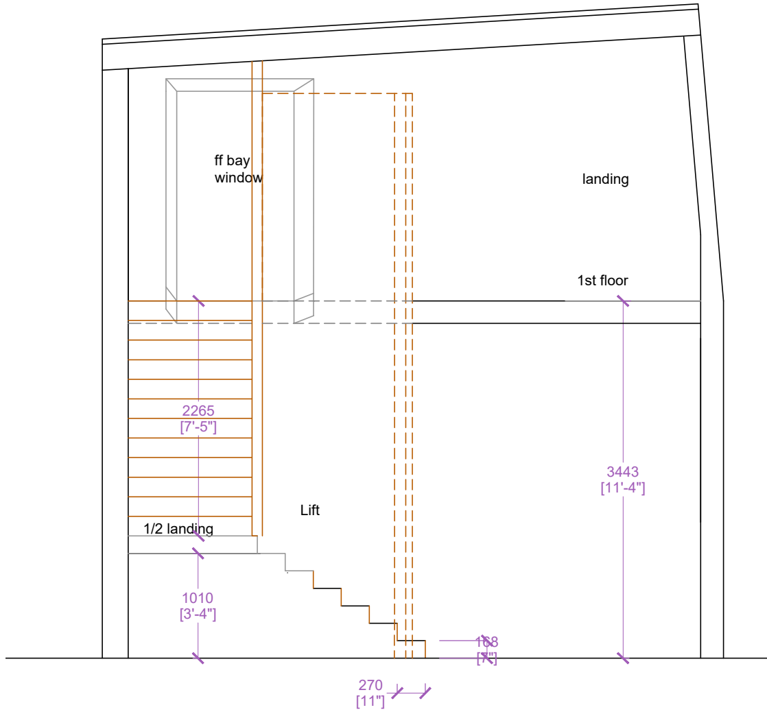
Proposed new stair section A-A
